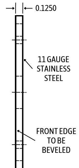
SIDE VIEW SS FACE PLATE
